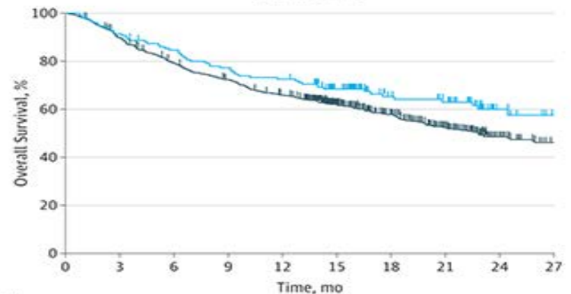
Overall survival
