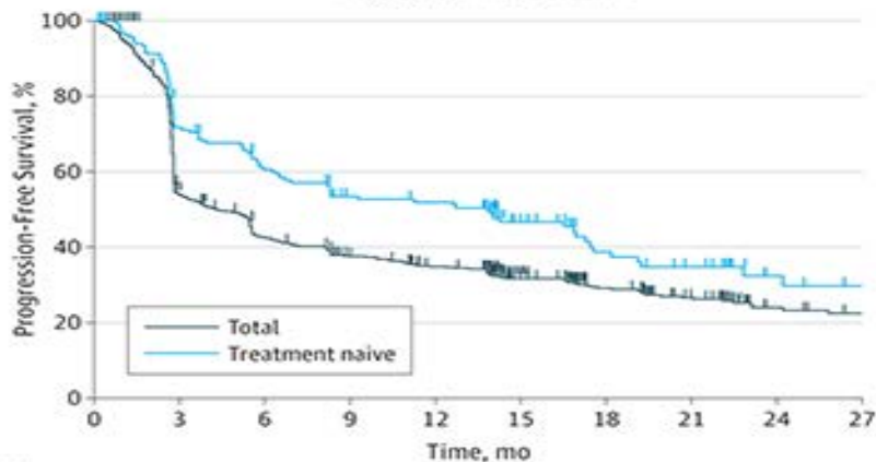
Progression-free survival
